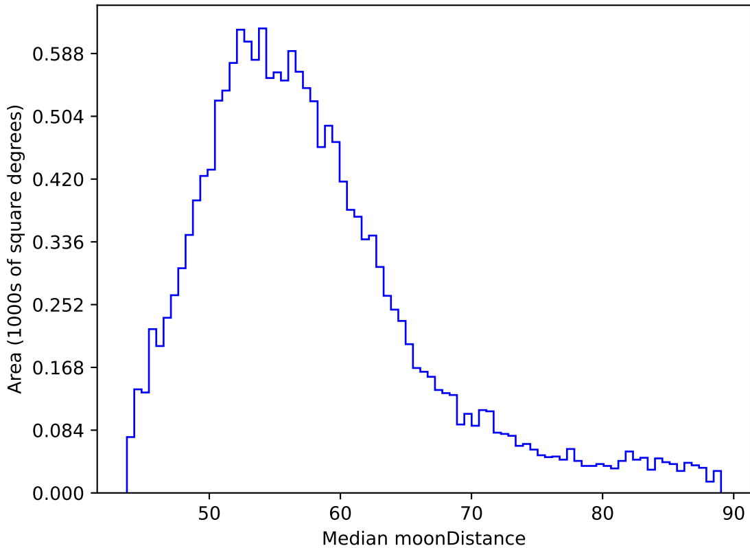
ddf_acor_sf10_lsf20_lsr50_v3.4_10yrs WFD y band: Median moonDistance
