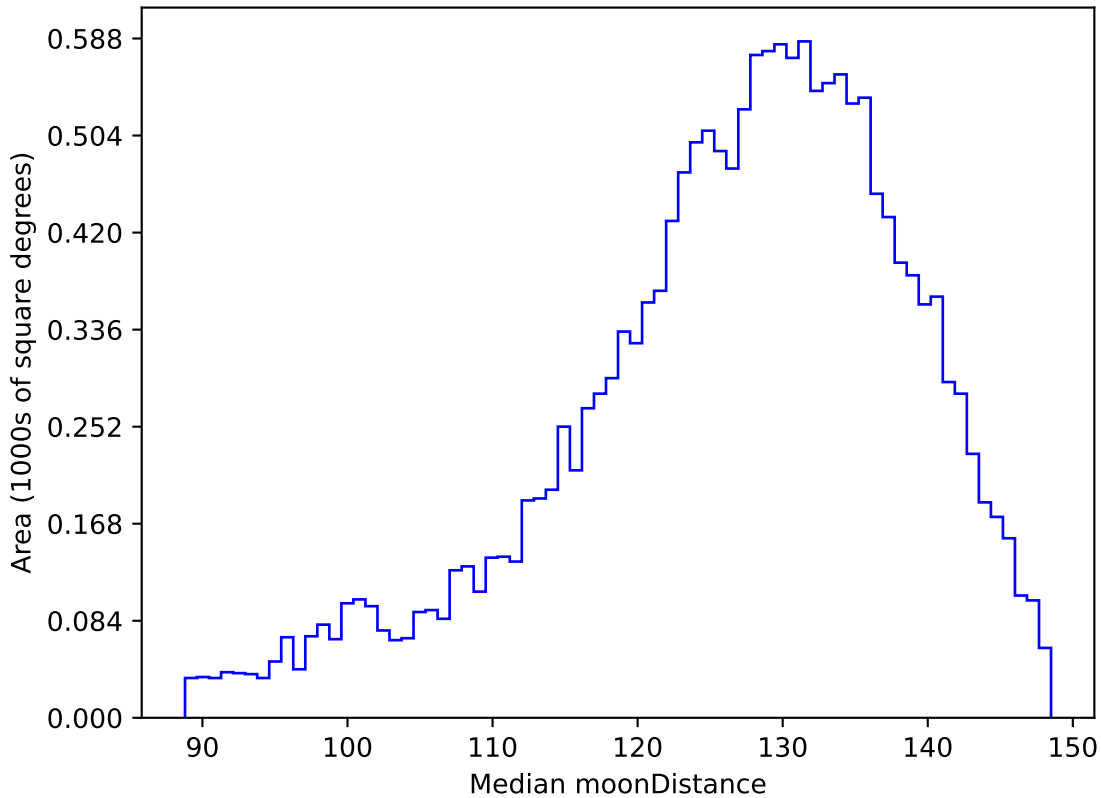
ddf_acor_sf10_ls20_lsr50_v3.4_10yrs WFD u band: Median moonDistance
