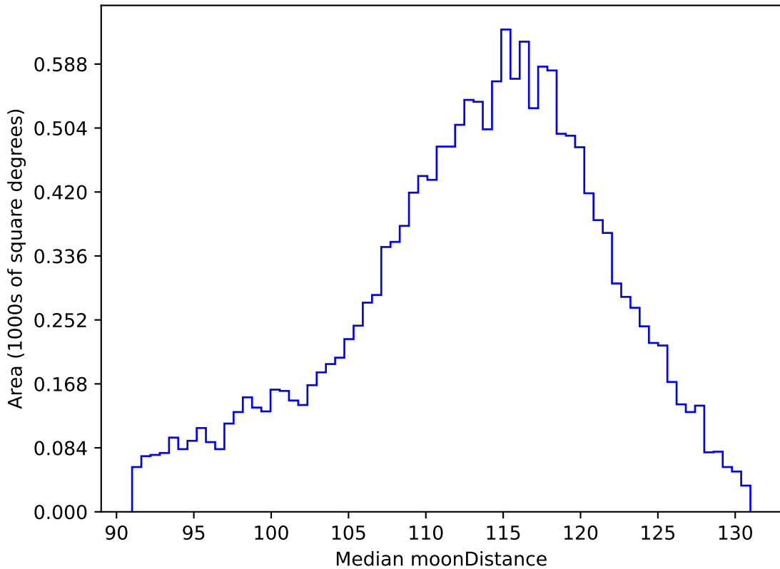
ddf_acor_sf10_lsf20_lsr50_v3.4_10yrs WFD r band: Median moonDistance
