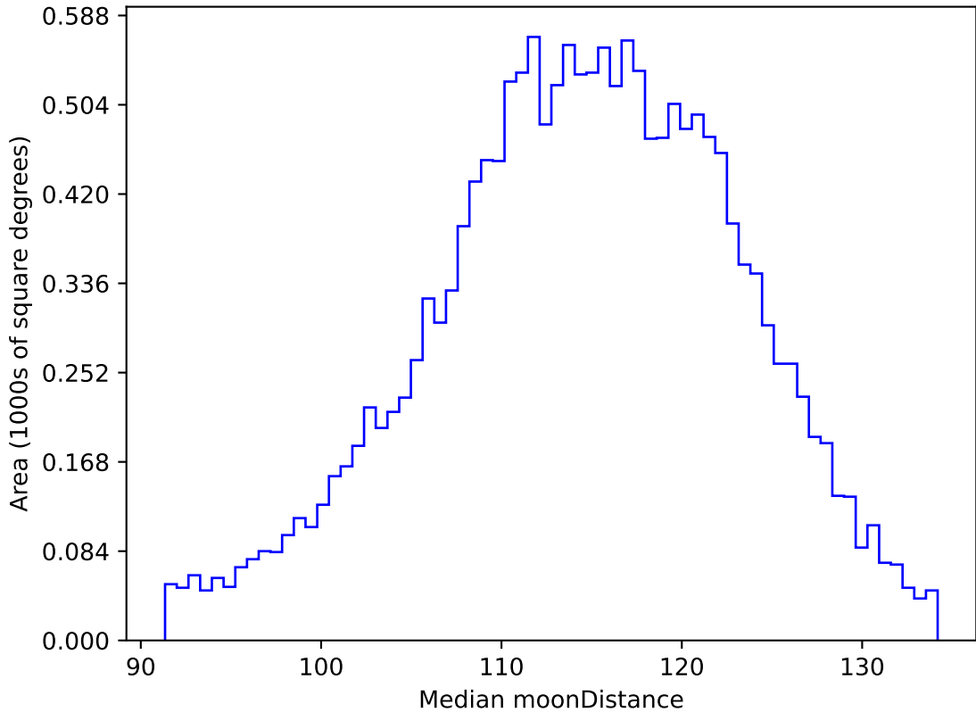
ddf_acor_sf10_lsf20_lsr50_v3.4_10yrs WFD g band: Median moonDistance
