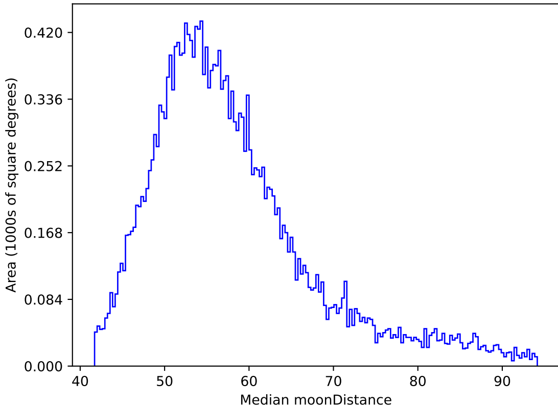
ddf_acor_sf10_lsf20_lsr50_v3.4_10yrs All sky y band: Median moonDistance
