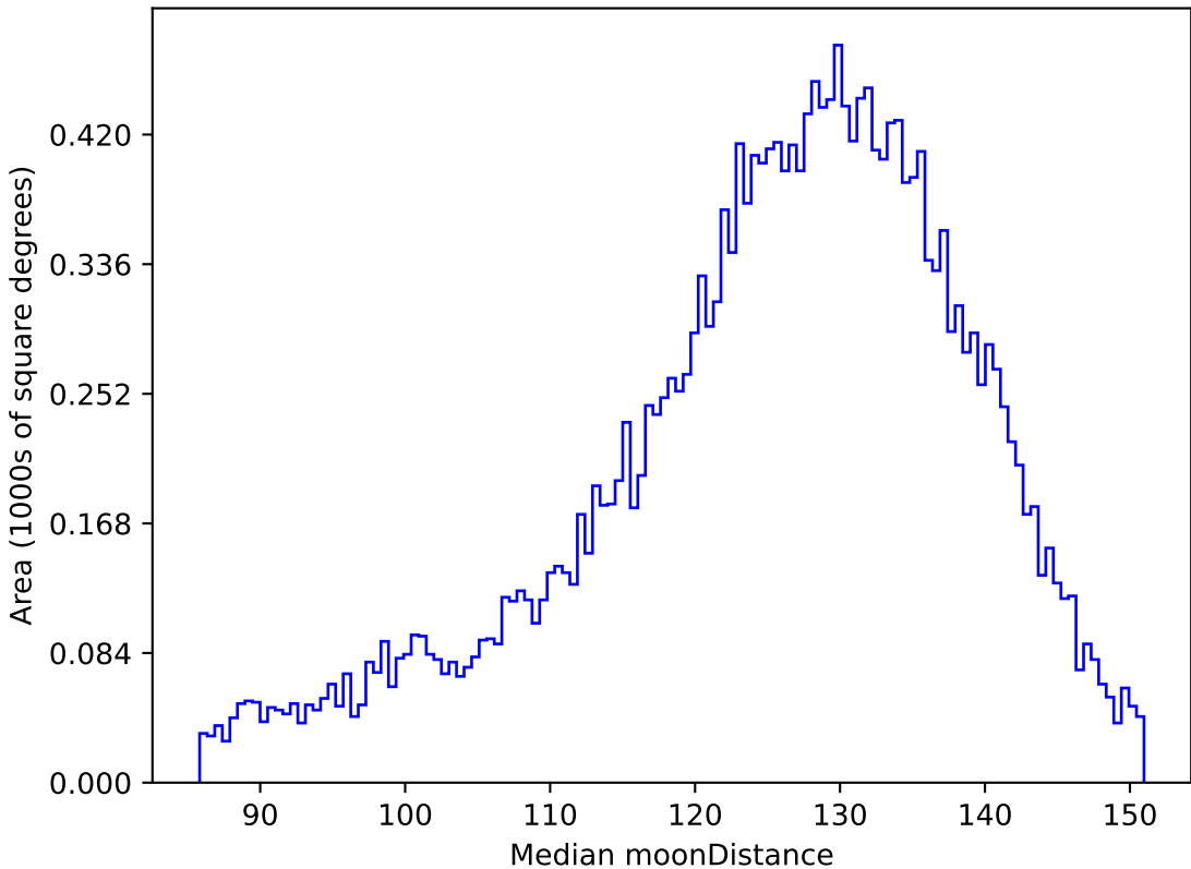
ddf_acor_sf10_lsf20_lsr50_v3.4_10yrs All sky u band: Median moonDistance
