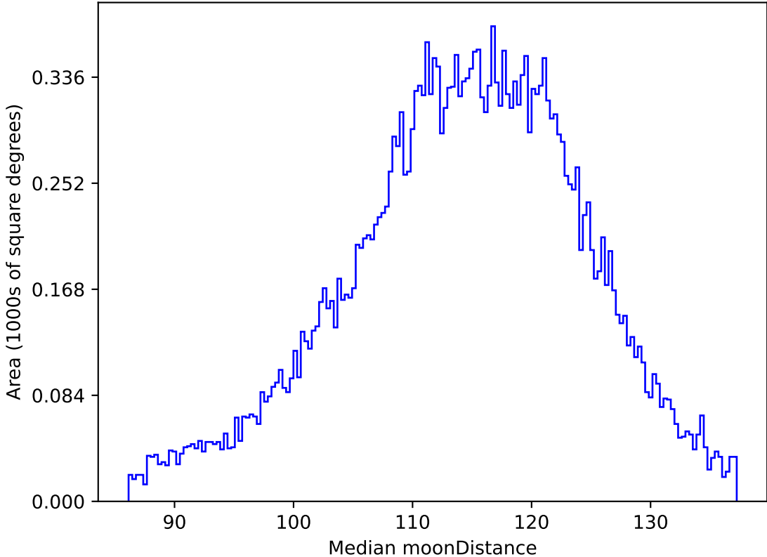
ddf_acor_sf10_lsf20_lsr50_v3.4_10yrs All sky g band: Median moonDistance
