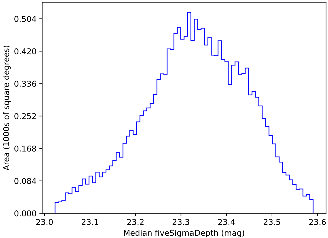
ddf_acor_sf10_lsf20_lsr50_v3.4_10yrs WFD all bands: Median fiveSigmaDepth
