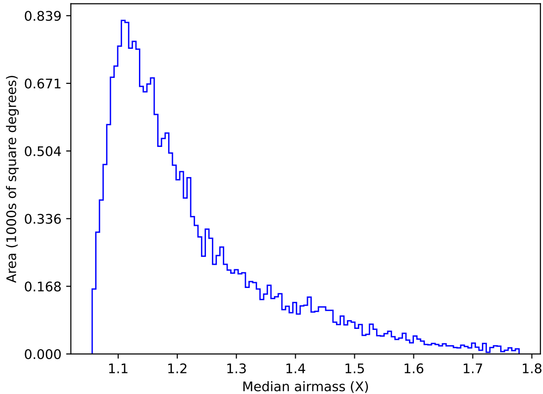
ddf_acor_sf10_lsf20_lsr50_v3.4_10yrs Yr 1 u band: Median airmass
