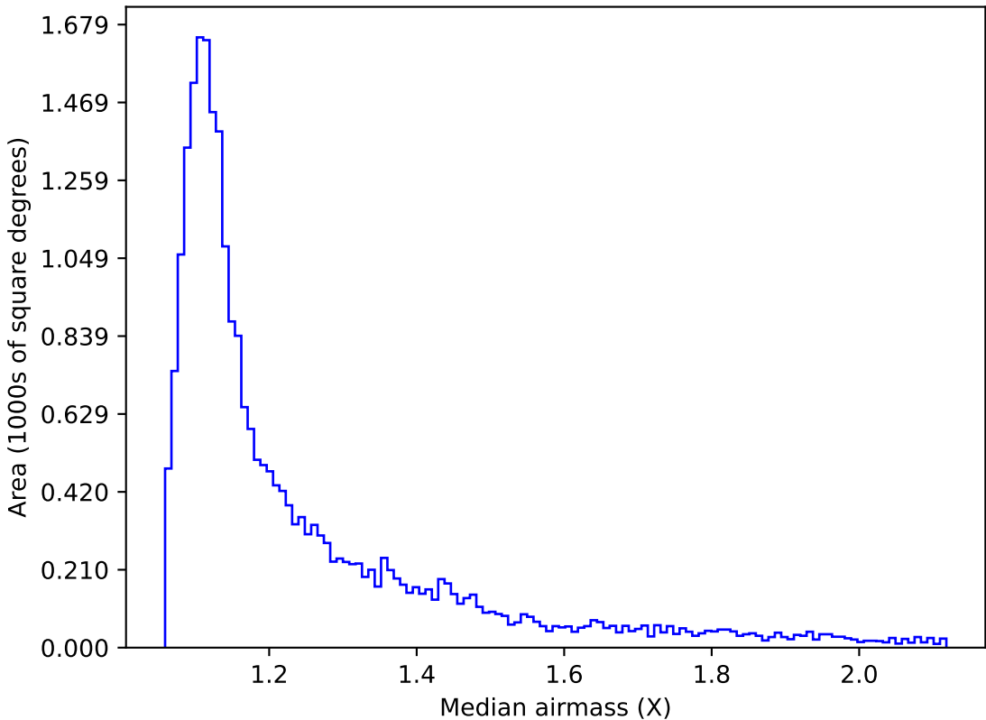
ddf_acor_sf10_lsf20_lsr50_v3.4_10yrs Yr 1 r band: Median airmass
