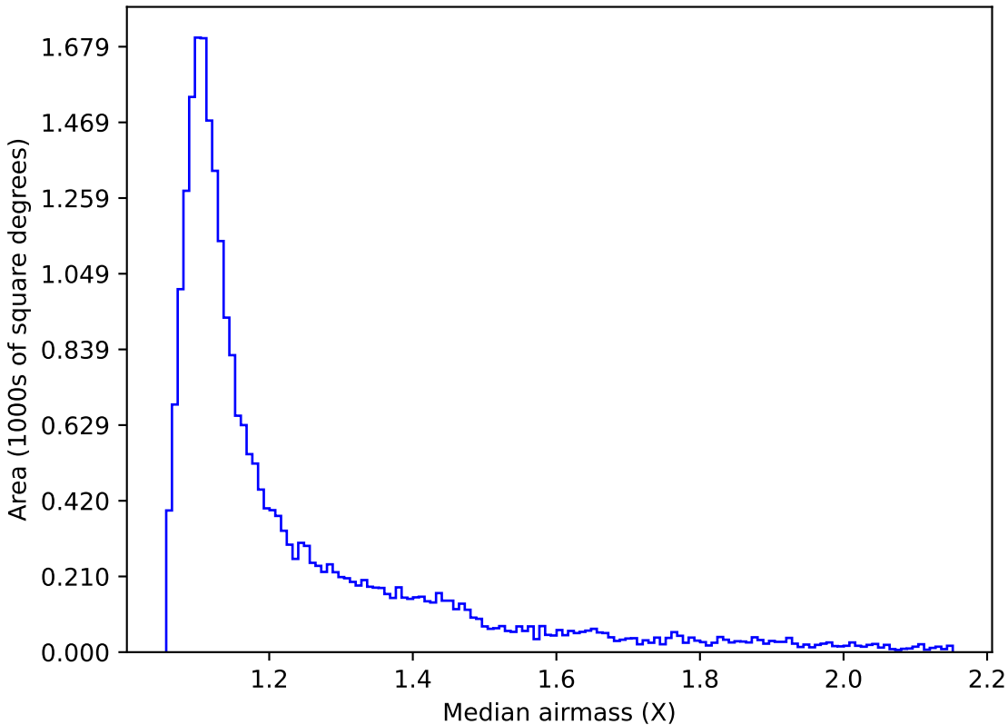
ddf_acor_sf10_lsf20_lsr50_v3.4_10yrs Yr 1 i band: Median airmass
