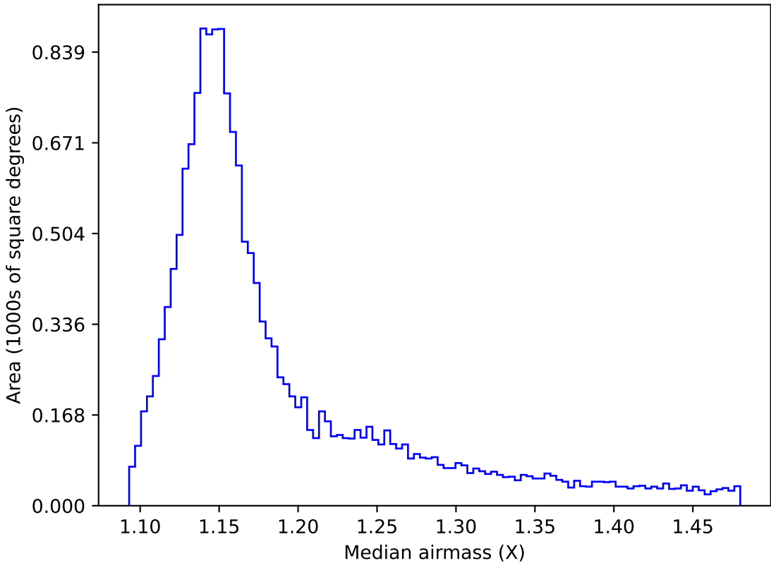
ddf_acor_sf10_lsf20_lsr50_v3.4_10yrs WFD y band: Median airmass
