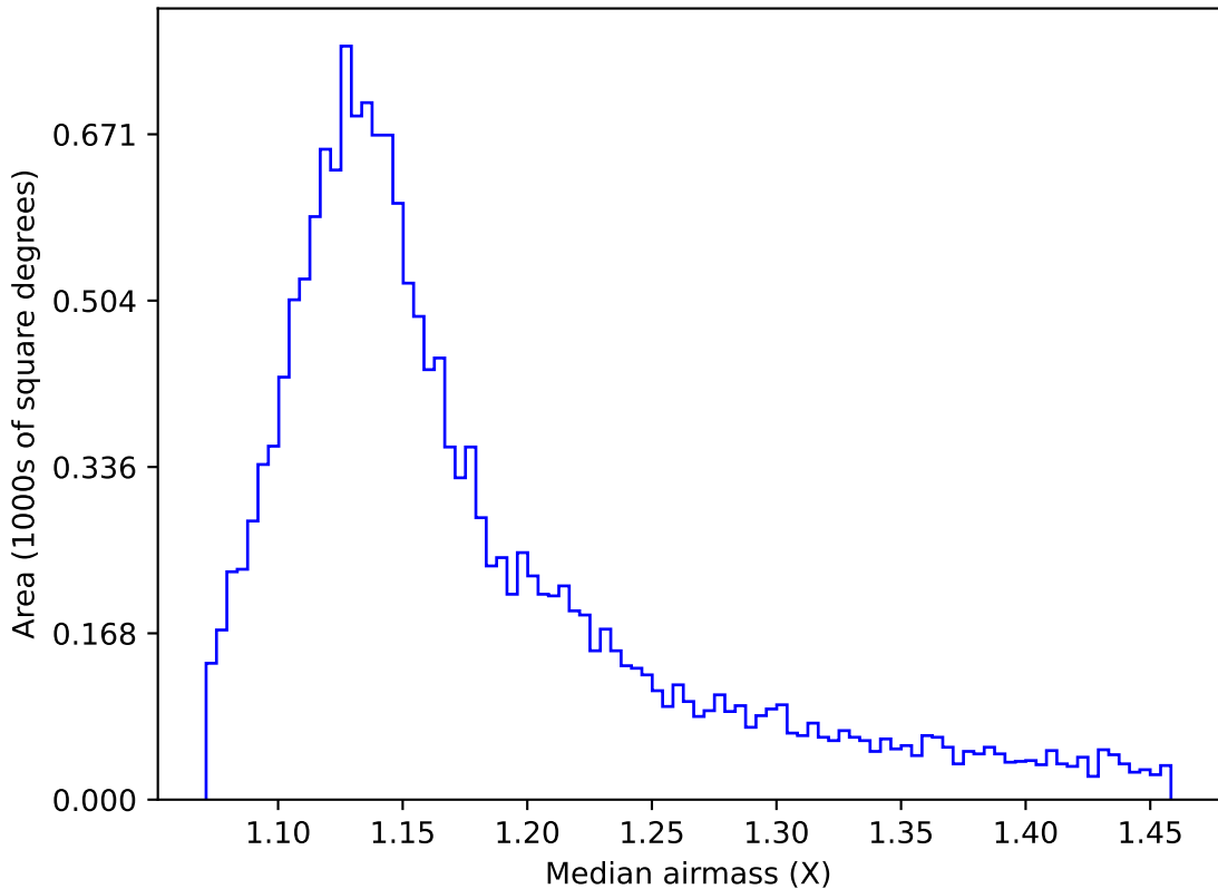
ddf_acor_sf10_lsf20_lsr50_v3.4_10yrs WFD u band: Median airmass
