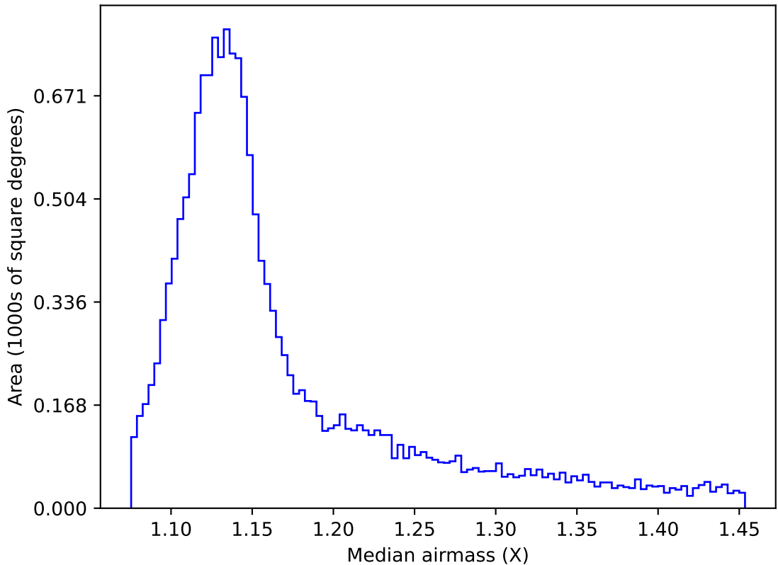
ddf_acor_sf10_lsf20_lsr50_v3.4_10yrs WFD i band: Median airmass
