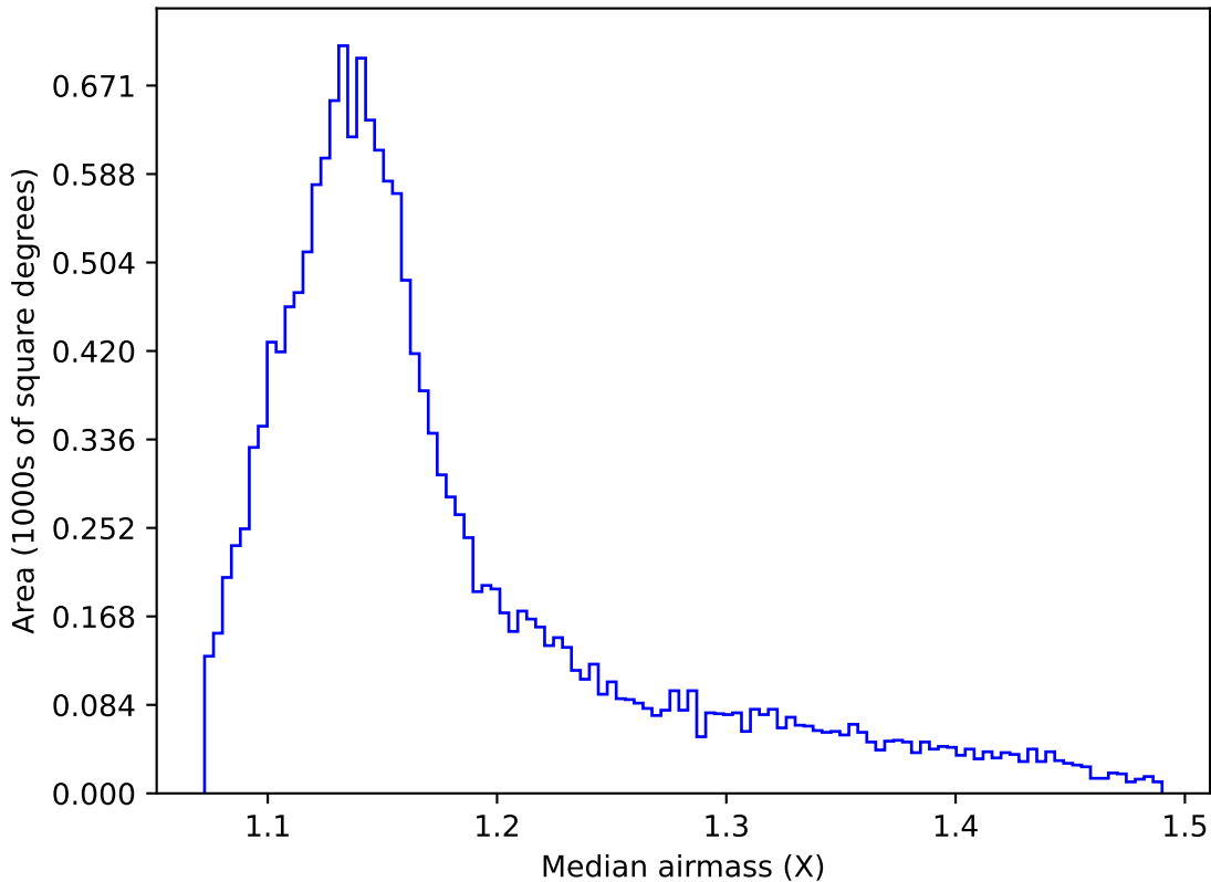
ddf_acor_sf10_lsf20_lsr50_v3.4_10yrs WFD g band: Median airmass
