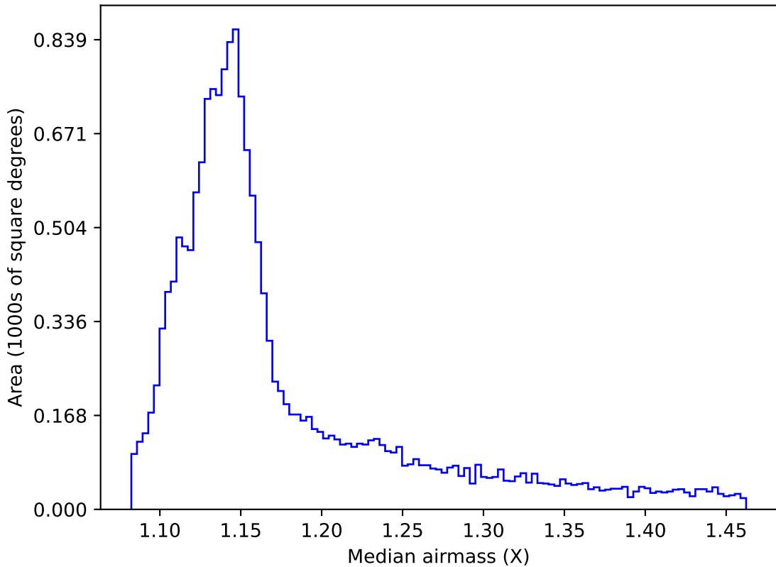
ddf_acor_sf10_lsf20_lsr50_v3.4_10yrs WFD all bands: Median airmass
