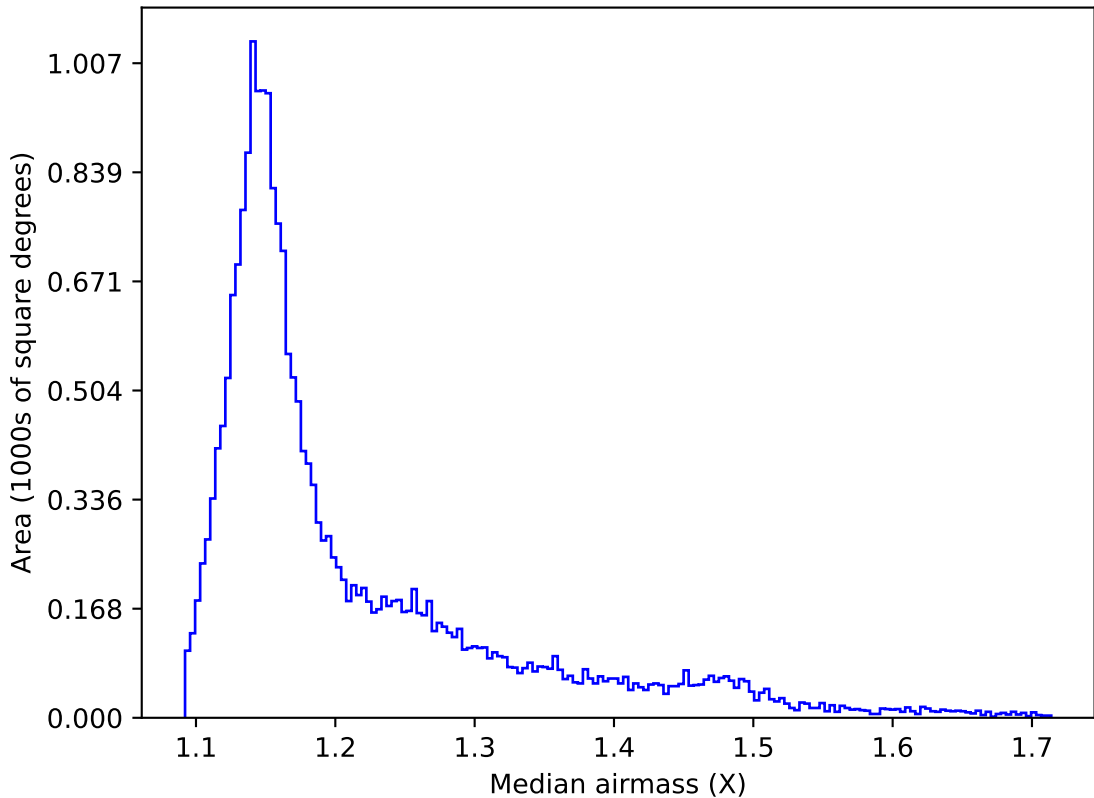
ddf_acor_sf10_lsf20_lsr50_v3.4_10yrs All sky y band: Median airmass
