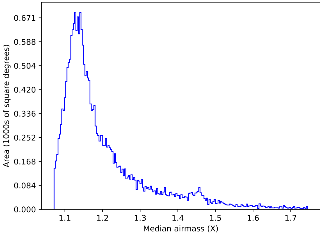
ddf_acor_sf10_lsf20_lsr50_v3.4_10yrs All sky u band: Median airmass
