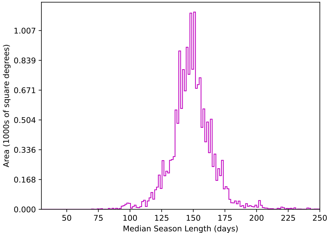
ddf_acor_sf10_lsf20_lsr50_v3.4_10yrs WFD z band: Median Season Length
