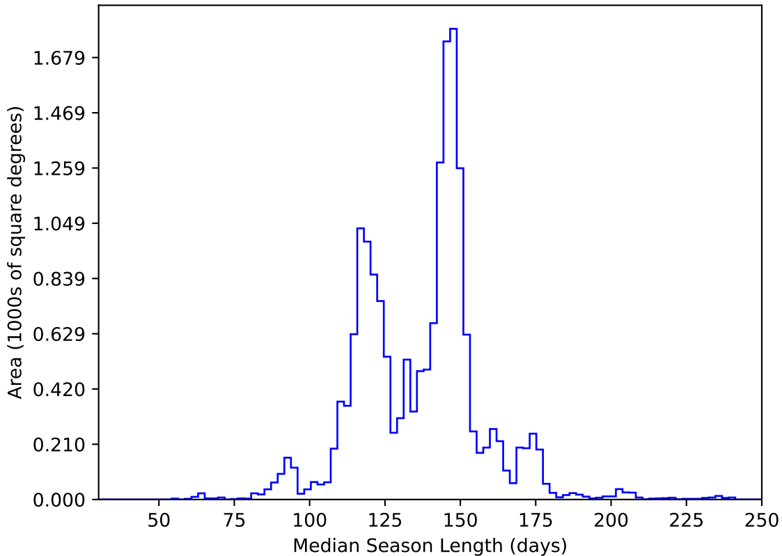
ddf_acor_sf10_lsf20_lsr50_v3.4_10yrs WFD y band: Median Season Length
