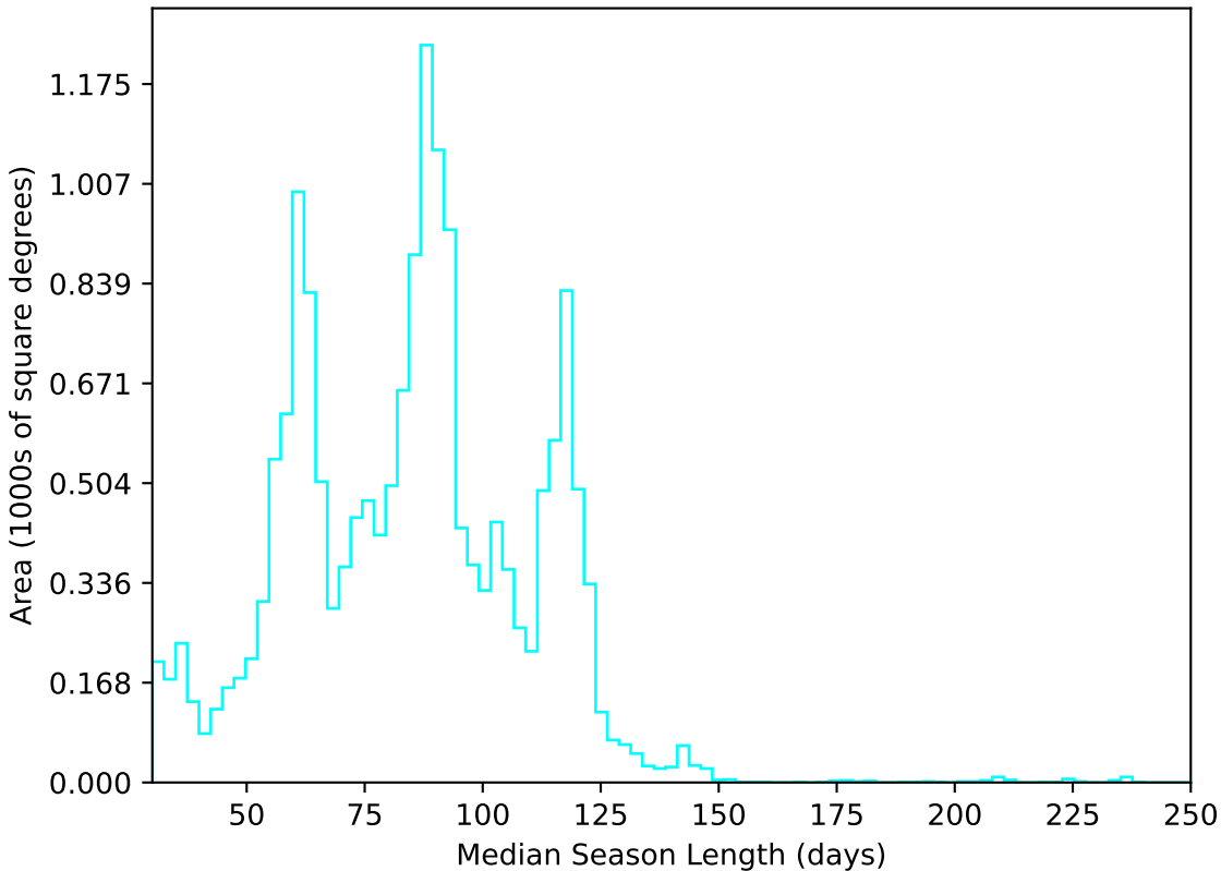
ddf_acor_sf10_lsf20_lsr50_v3.4_10yrs WFD u band: Median Season Length
