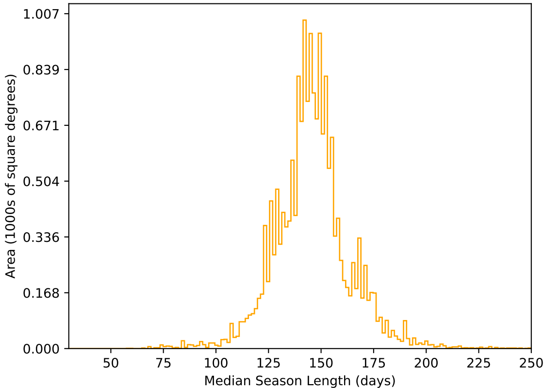
ddf_acor_sf10_lsf20_lsr50_v3.4_10yrs WFD r band: Median Season Length
