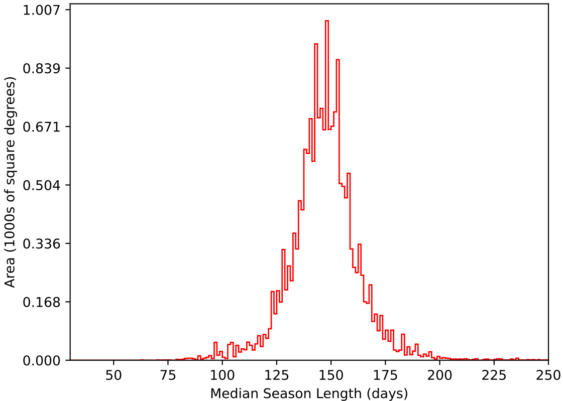
ddf_acor_sf10_lsf20_lsr50_v3.4_10yrs WFD i band: Median Season Length
