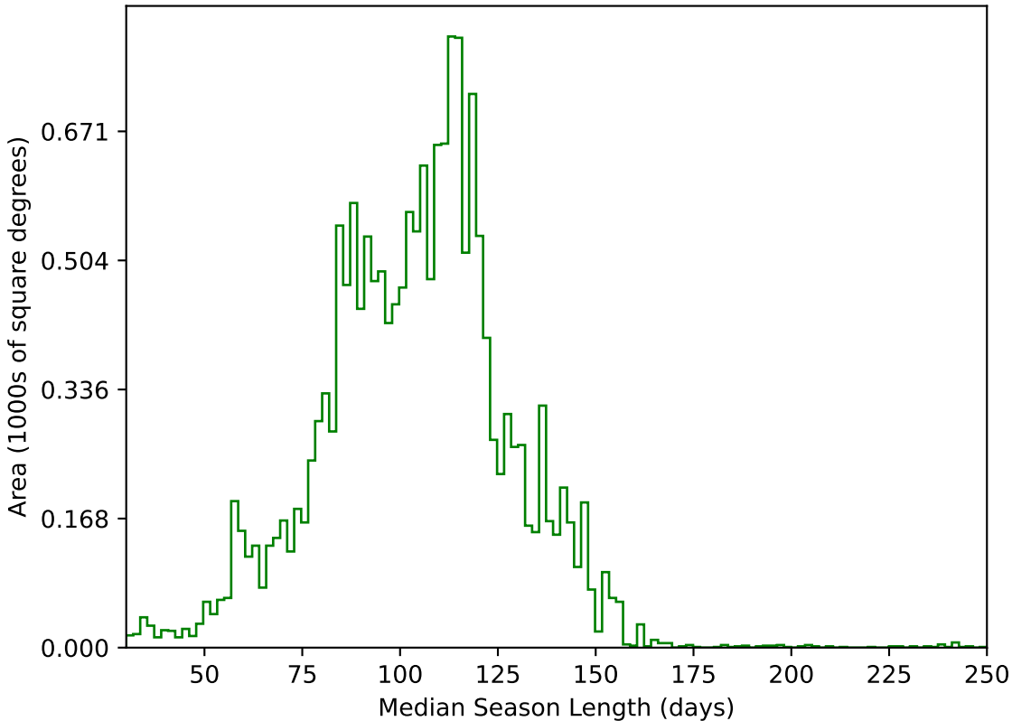
ddf_acor_sf10_ls20_lsr50_v3.4_10yrs WFD g band: Median Season Length
