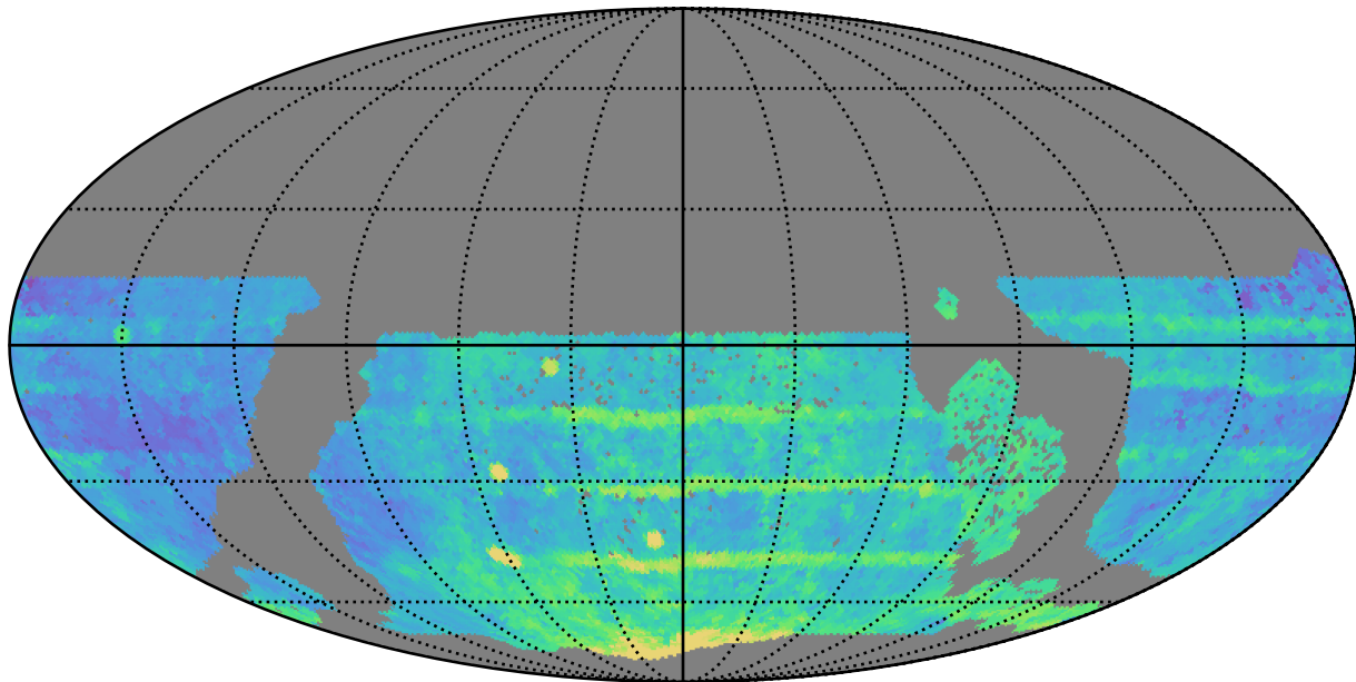
ddf_acor_sf10_lsf20_lsr50_v3.4_10yrs WFD all bands: Median Season Length
