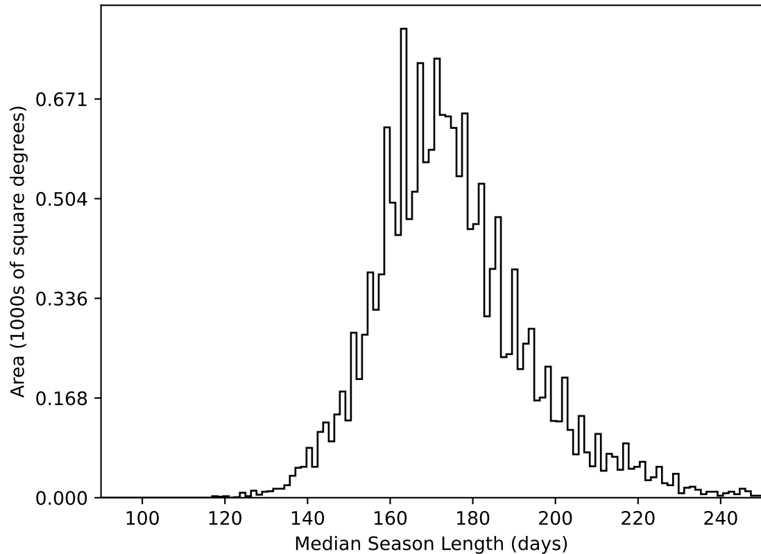
ddf_acor_sf10_lsf20_lsr50_v3.4_10yrs WFD all bands: Median Season Length
