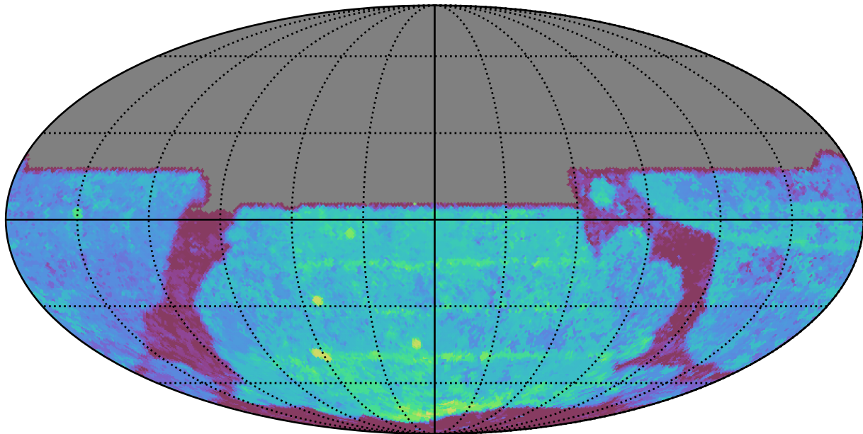
ddf_acor_sf10_lsf20_lsr50_v3.4_10yrs All sky y band: Median Season Length
