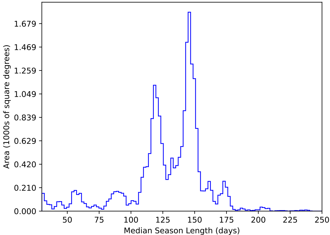
ddf_acor_sf10_lsf20_lsr50_v3.4_10yrs All sky y band: Median Season Length
