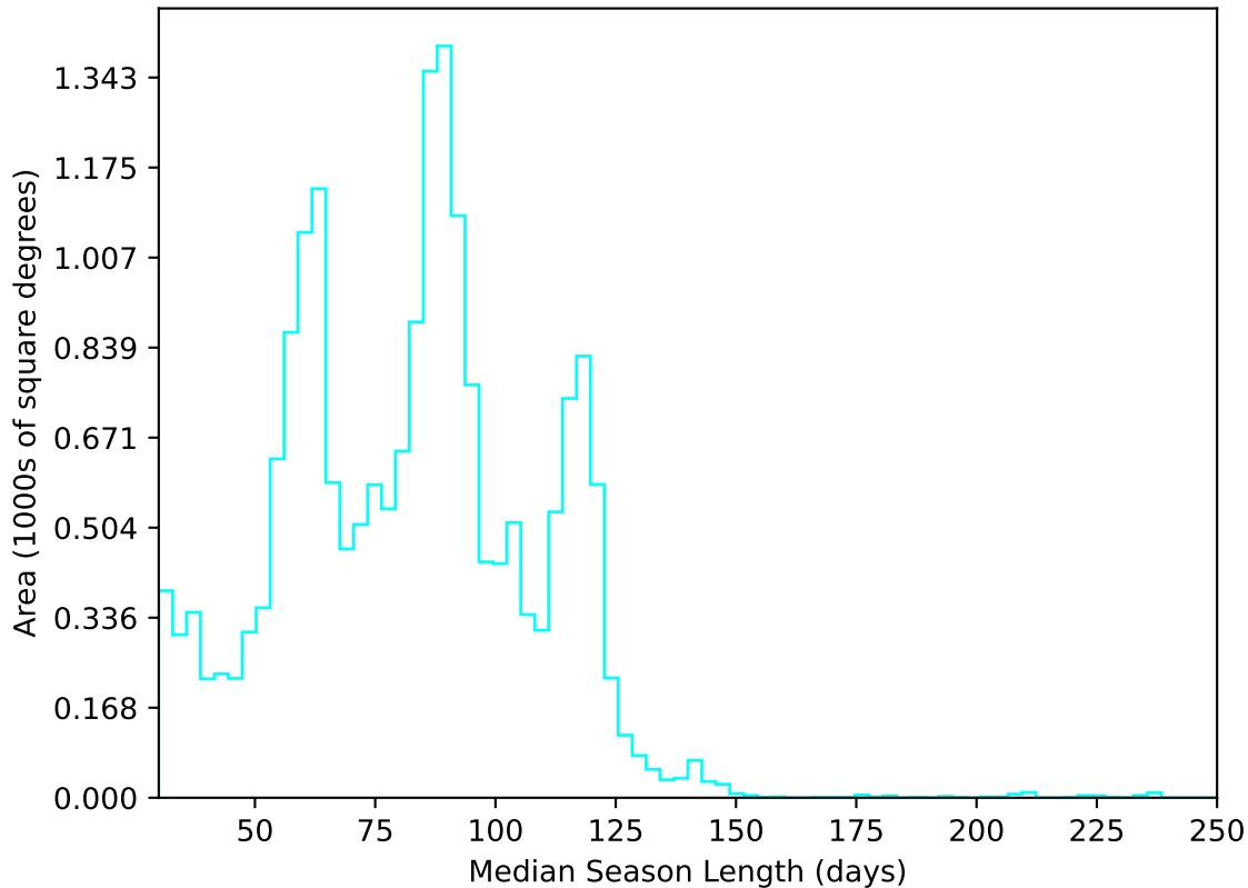
ddf_acor_sf10_lsf20_lsr50_v3.4_10yrs All sky u band: Median Season Length
