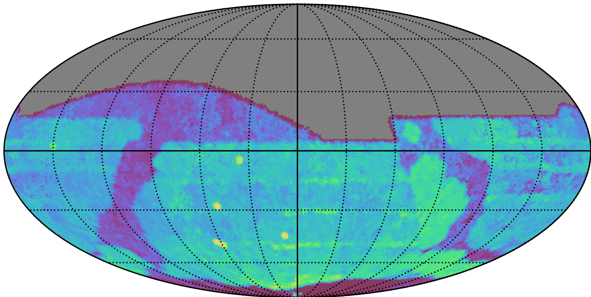
ddf_acor_sf10_lsf20_lsr50_v3.4_10yrs All sky r band: Median Season Length
