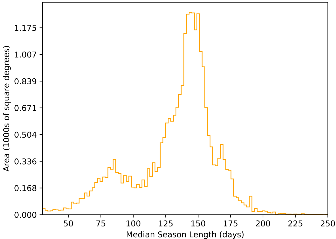
ddf_acor_sf10_lsf20_lsr50_v3.4_10yrs All sky r band: Median Season Length
