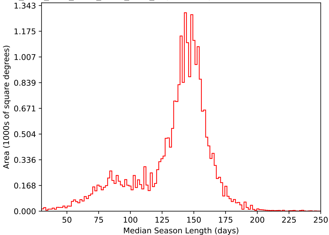
ddf_acor_sf10_lsf20_lsr50_v3.4_10yrs All sky i band: Median Season Length
