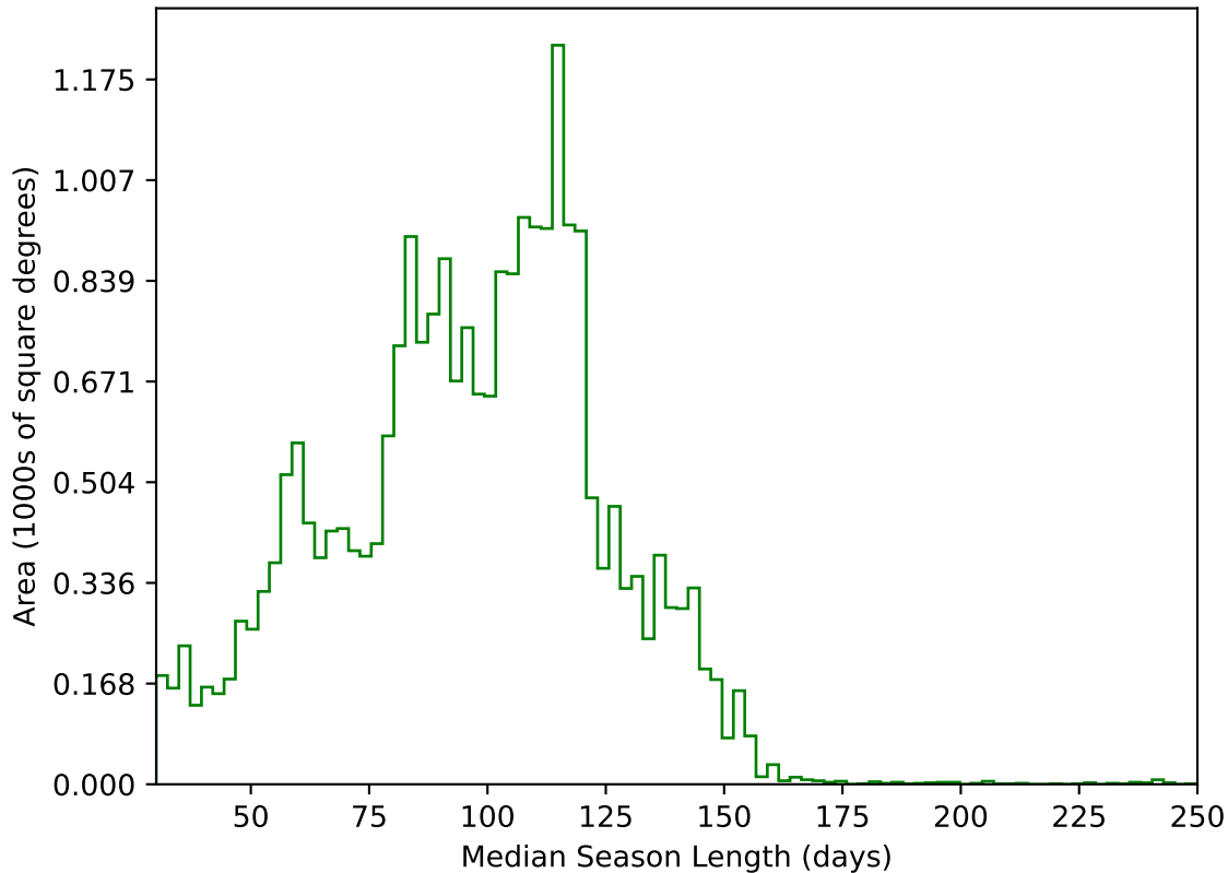
ddf_acor_sf10_lsf20_lsr50_v3.4_10yrs All sky g band: Median Season Length
