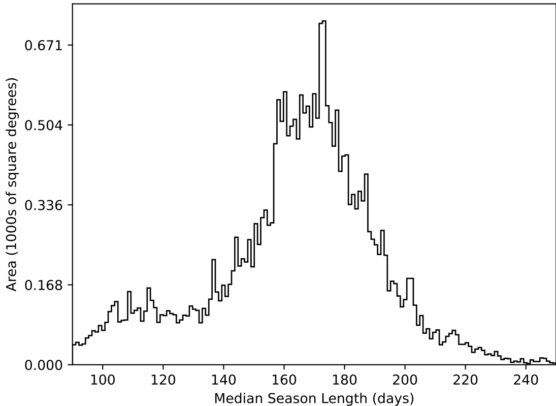
ddf_acor_sf10_lsf20_lsr50_v3.4_10yrs All sky all bands: Median Season Length
