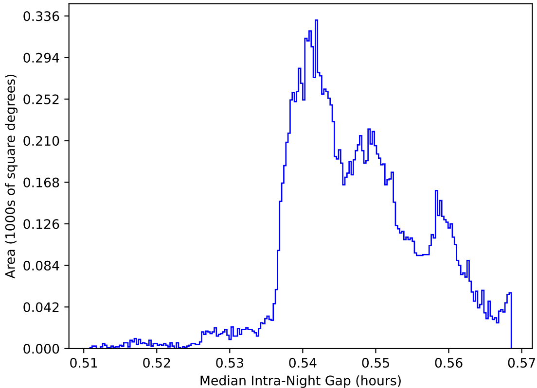
ddf_acor_sf10_lsf20_lsr50_v3.4_10yrs WFD: Median Intra-Night Gap
