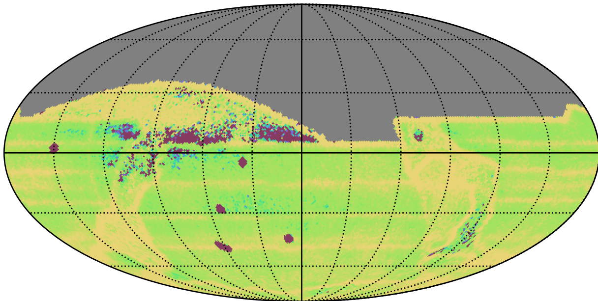
ddf_acor_sf10_lsf20_lsr50_v3.4_10yrs All sky: Median Intra-Night Gap
