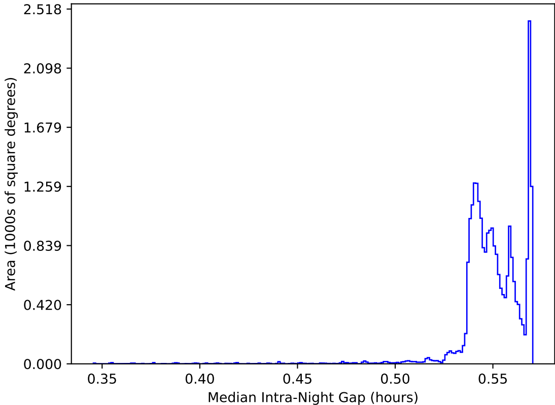
ddf_acor_sf10_lsf20_lsr50_v3.4_10yrs All sky: Median Intra-Night Gap
