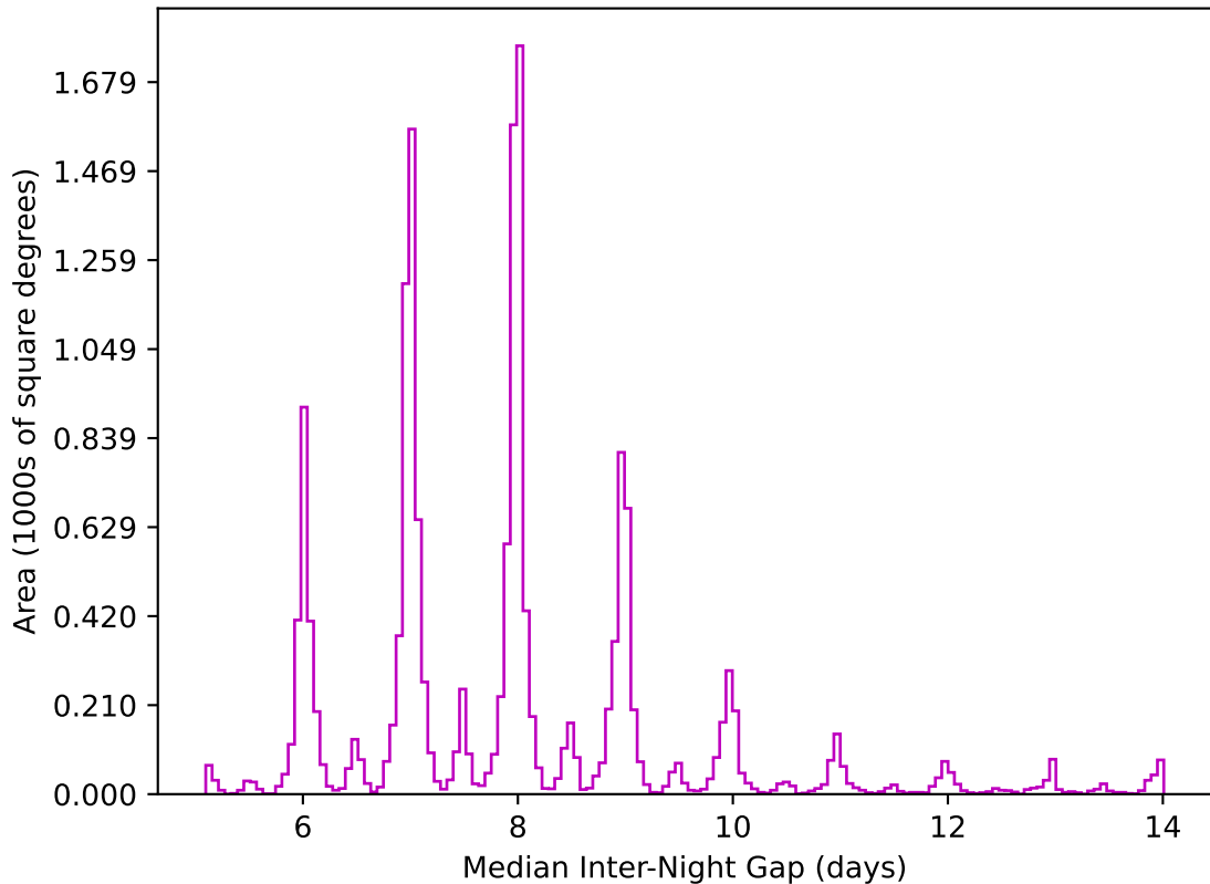
ddf_acor_sf10_lsf20_lsr50_v3.4_10yrs WFD z band: Median Inter-Night Gap
