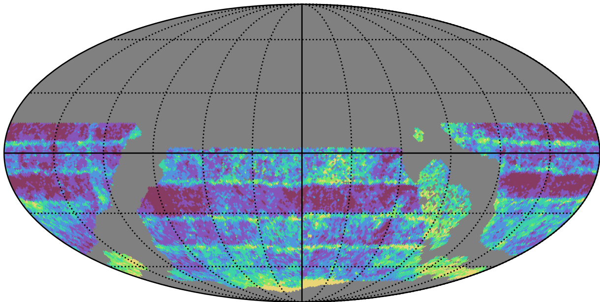
ddf_acor_sf10_lsf20_lsr50_v3.4_10yrs WFD r band: Median Inter-Night Gap
