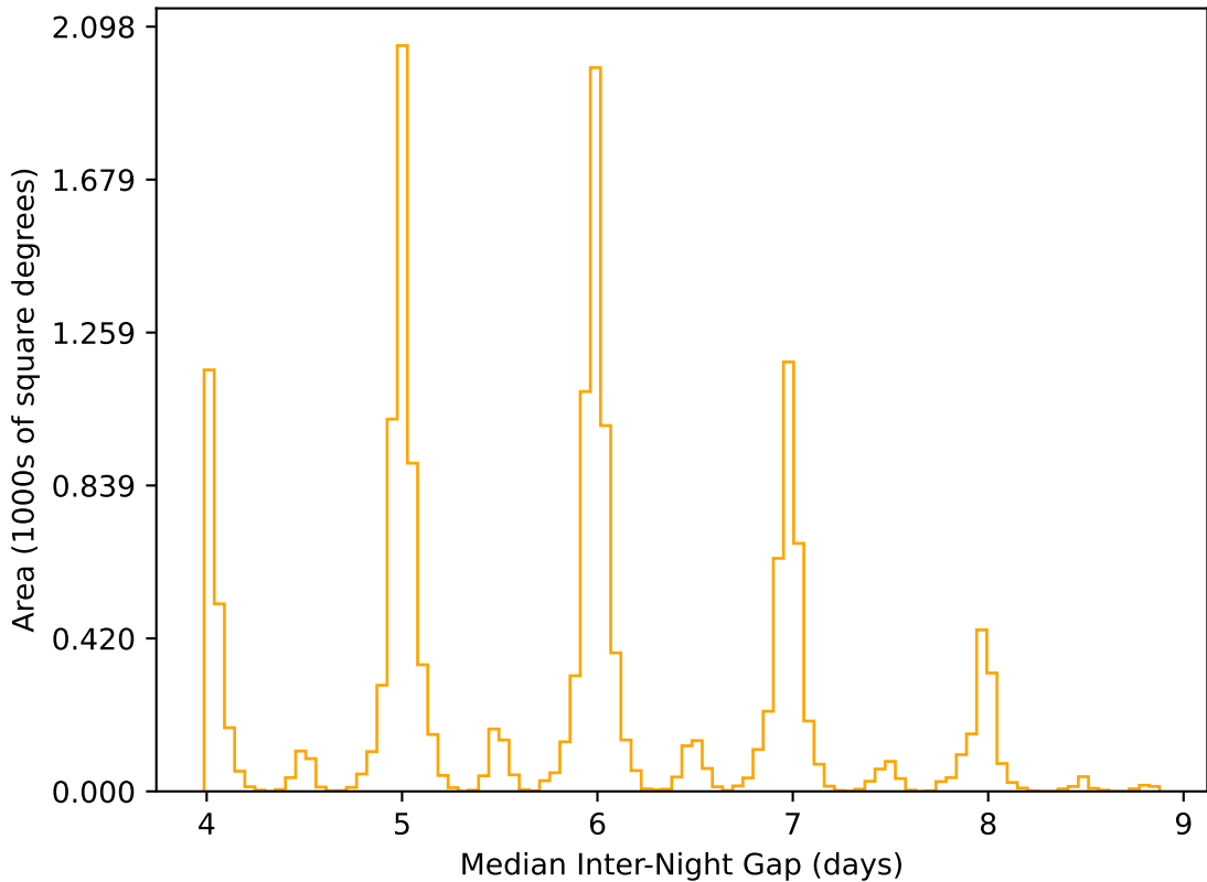
ddf_acor_sf10_ls20_lsr50_v3.4_10yrs WFD r band: Median Inter-Night Gap
