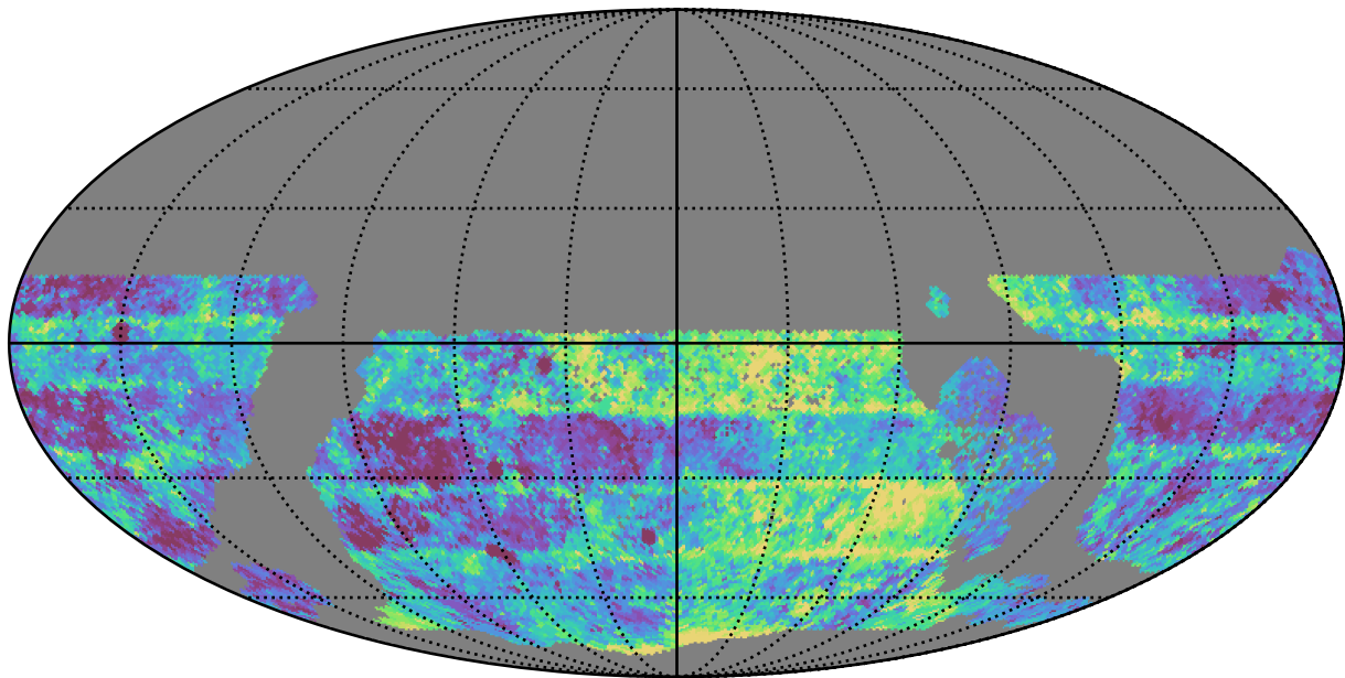
ddf_acor_sf10_lsf20_lsr50_v3.4_10yrs WFD g band: Median Inter-Night Gap
