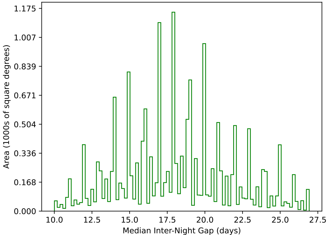
ddf_acor_sf10_lsf20_lsr50_v3.4_10yrs WFD g band: Median Inter-Night Gap
