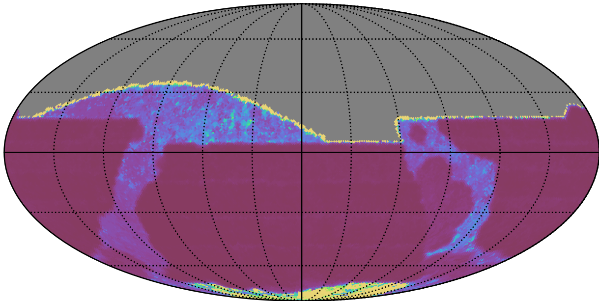
ddf_acor_sf10_lsf20_lsr50_v3.4_10yrs All sky z band: Median Inter-Night Gap
