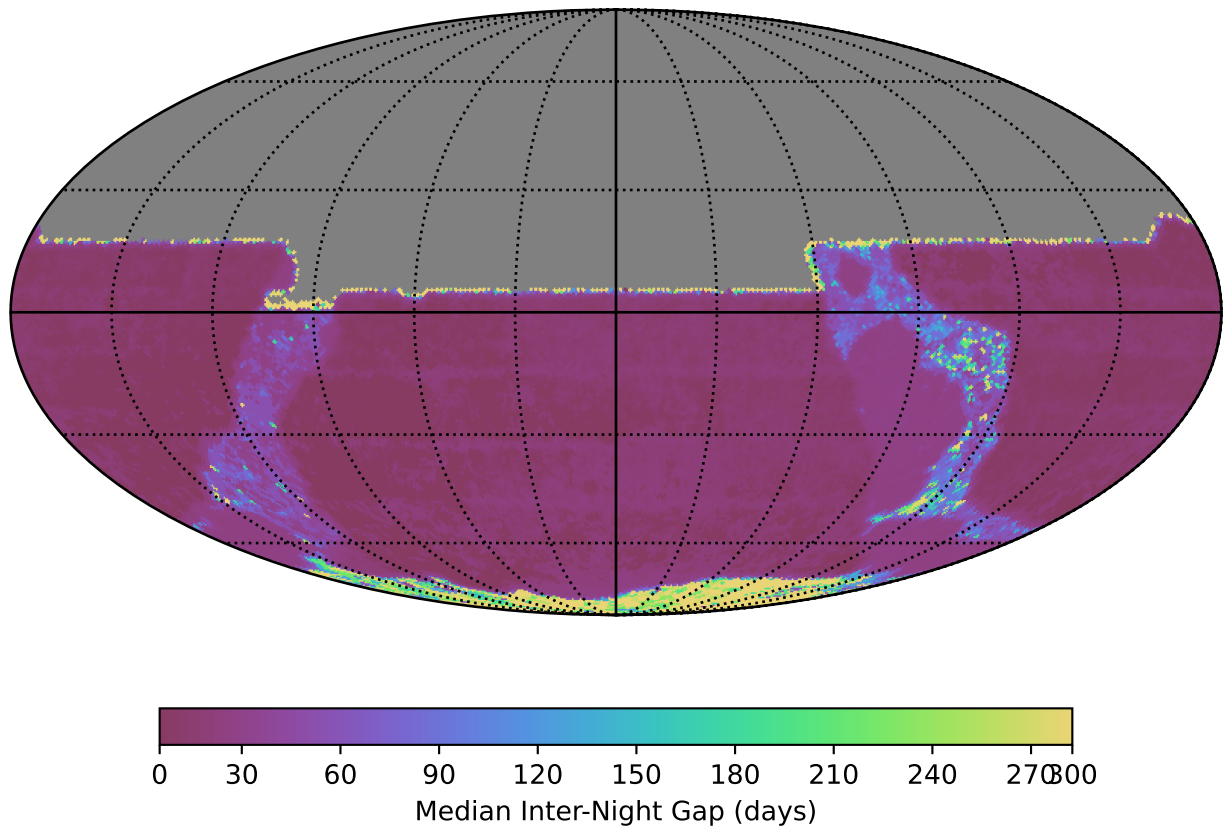
ddf_acor_sf10_lsf20_lsr50_v3.4_10yrs All sky y band: Median Inter-Night Gap
