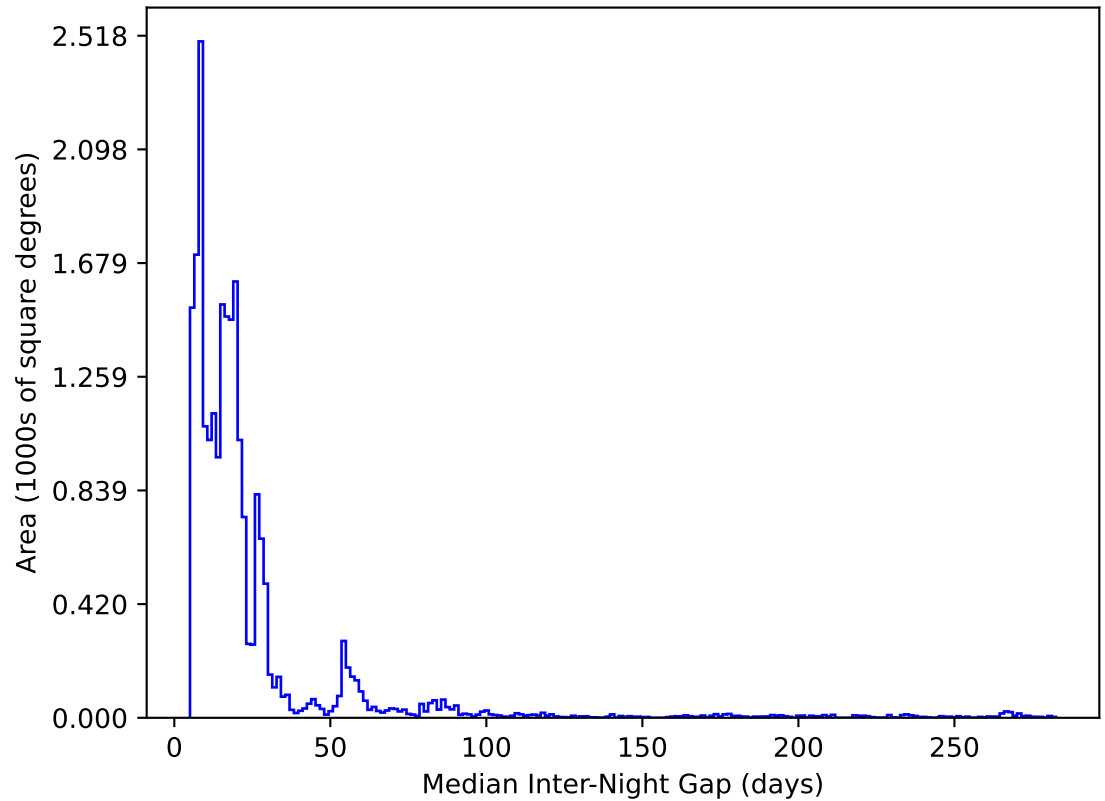
ddf_acor_sf10_lsf20_lsr50_v3.4_10yrs All sky y band: Median Inter-Night Gap
