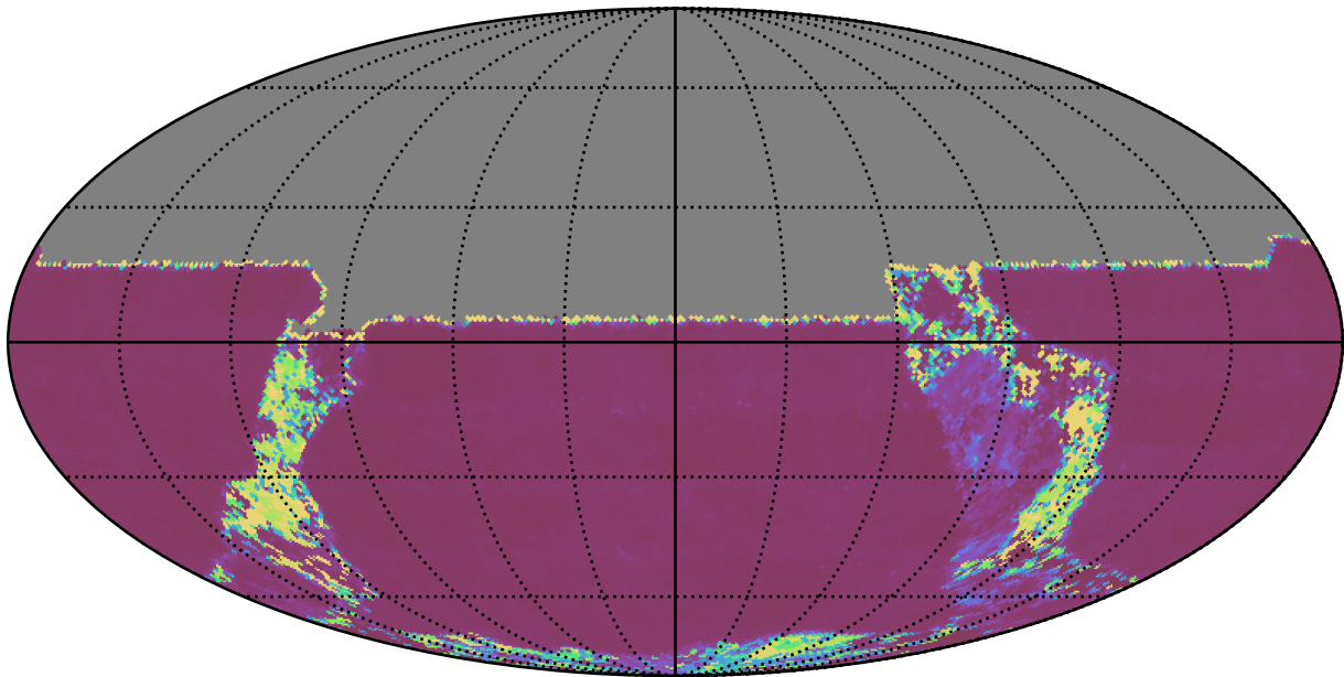
ddf_acor_sf10_lsf20_lsr50_v3.4_10yrs All sky u band: Median Inter-Night Gap
