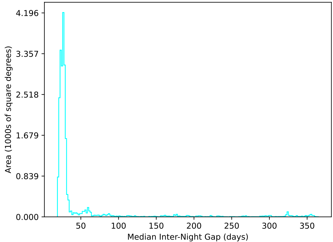
ddf_acor_sf10_lsf20_lsr50_v3.4_10yrs All sky u band: Median Inter-Night Gap
