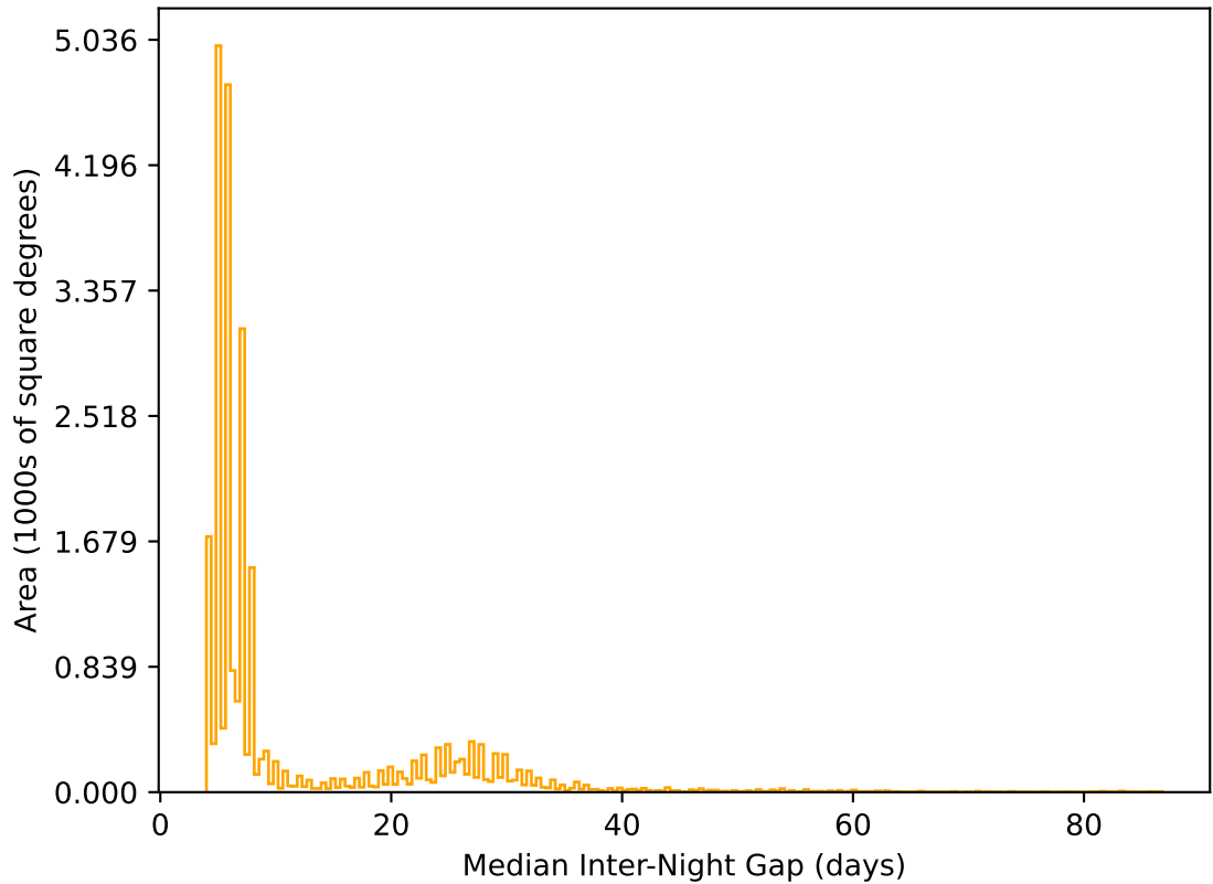
ddf_acor_sf10_lsf20_lsr50_v3.4_10yrs All sky r band: Median Inter-Night Gap
