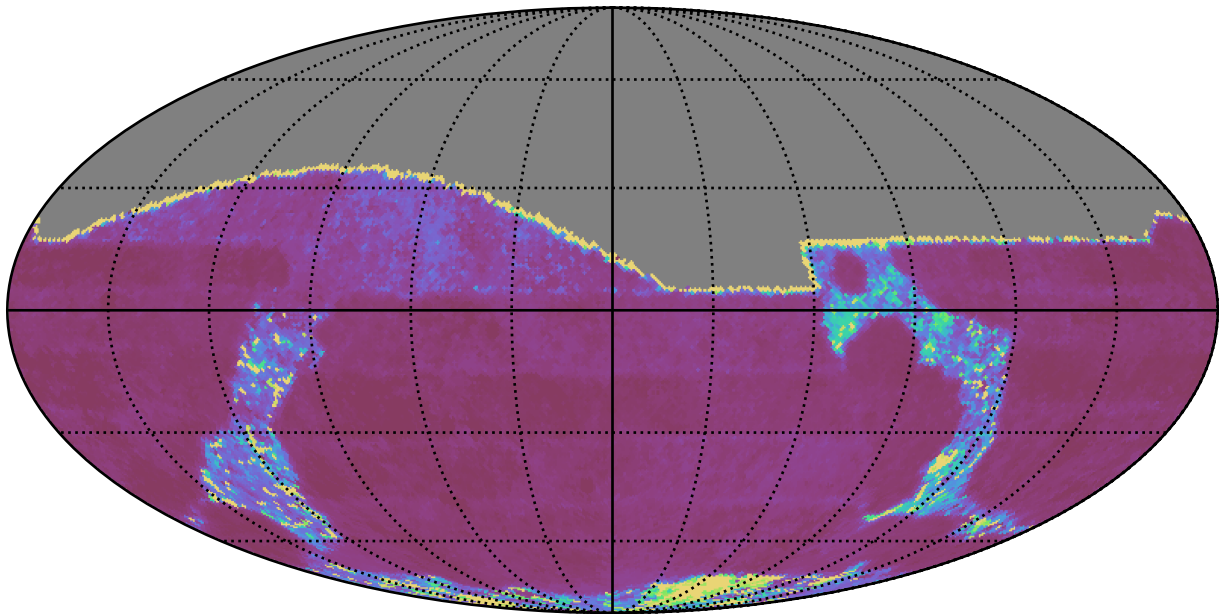
ddf_acor_sf10_lsf20_lsr50_v3.4_10yrs All sky g band: Median Inter-Night Gap
