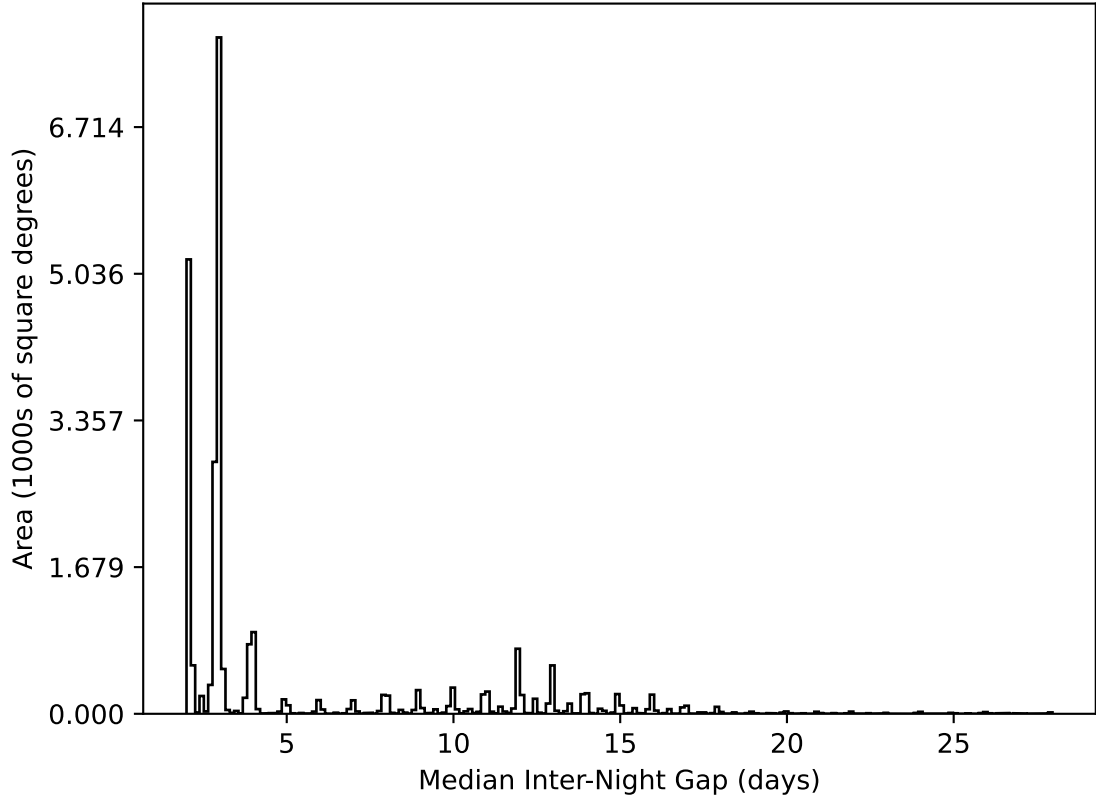
ddf_acor_sf10_lsf20_lsr50_v3.4_10yrs All sky all bands: Median Inter-Night Gap
